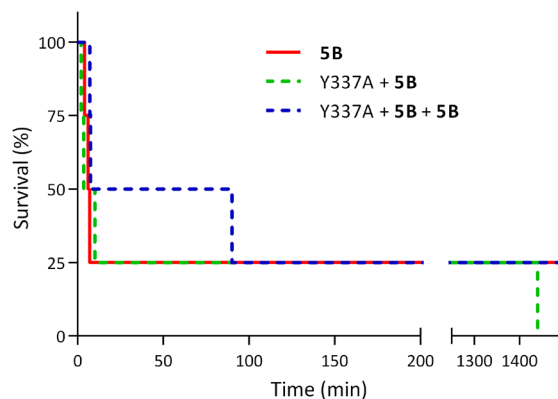
Fig. 2. Survival plots for mice exposed to 2 x LD 50 of tabun ( s.c. ). All of the groups received oxime 5B (40 mg/kg equals 0.25 of its LD 50 ; i.m. ) in atropine (10 mg/kg) 1 min after tabun exposure ( s.c. ). One group received additional dose of 5B (40 mg/kg; i.m. ) 30 min after the first administration. Two groups were pretreated with human AChE mutant Y337A (1 mg/kg, i.v. ) 15 min prior to tabun exposure ( s.c. ). LD 50 ( s.c. ) of tabun was 267 µg/kg. The experiment utilized four mice in each group.
